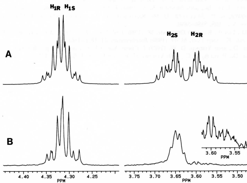
FIG. 2. Partial ^1H NMR spectra (500 MHz, CDCl_3 ) of N,O -dicamphanoyl-2-aminoethanols. A is from nonlabeled ethanolamine; B is compound 4 from deuterated ethanolamine as outlined in Fig. 1. The inset in B shows the residual signal with expanded y scale.
